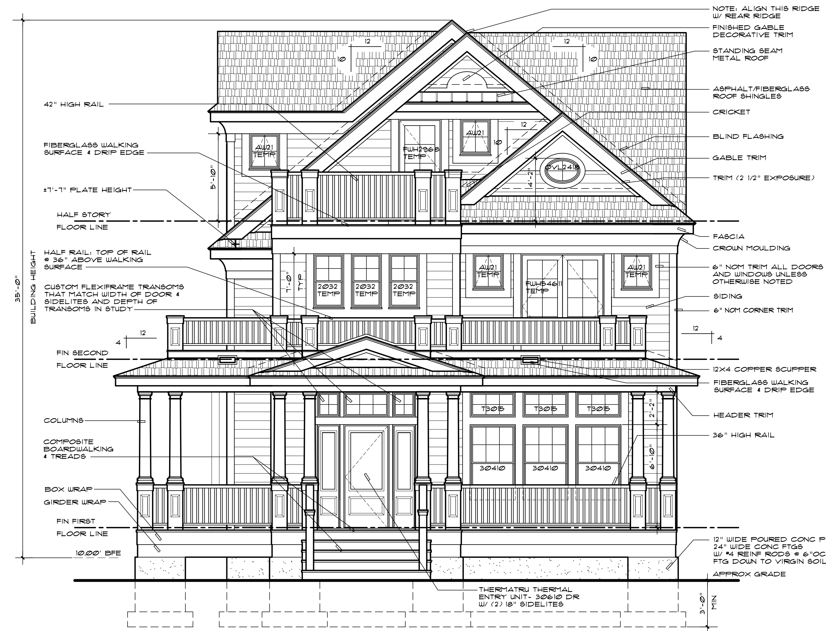
SOUTH ELEVATION
